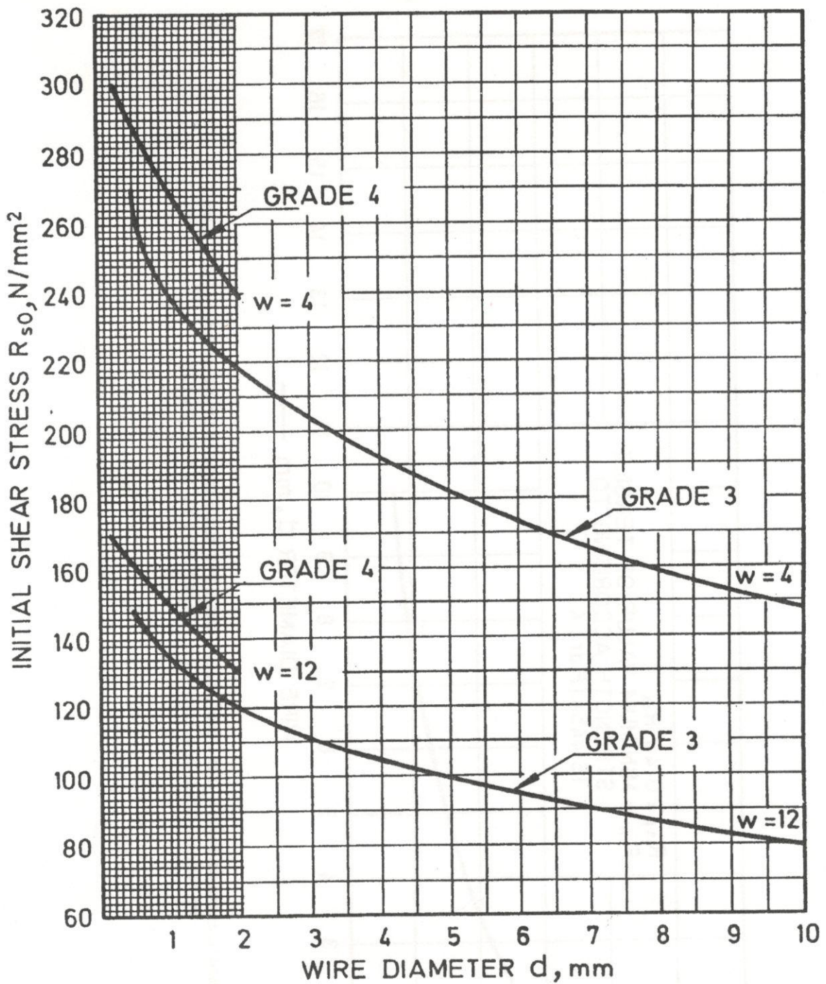
FIG. 7 HAND COILING — APPROXIMATE VALUES OF PERMISSIBLE INITIAL SHEAR STRESSES R_{50} FOR COLD COILED EXTENSION SPRINGS MADE FROM COLD DRAWN AND PATENTED SPRING STEEL WIRES OF GRADES 3 AND 4 TO IS 4454 (Part 1)
