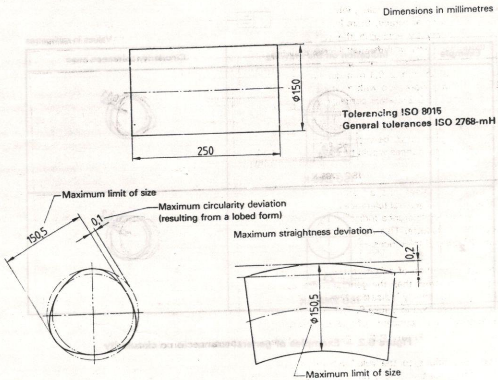
Figure B.1 — Principle of independency; maximum permissible deviations on the same feature
