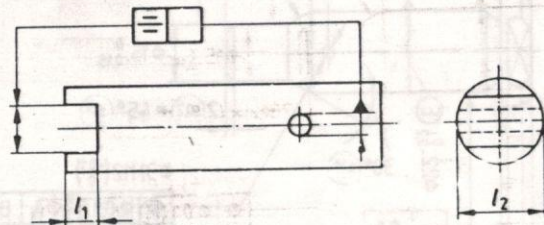
c) Datum: longer feature ( l_2 )
