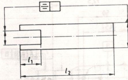
a) Datum: longer feature ( l_2 )
